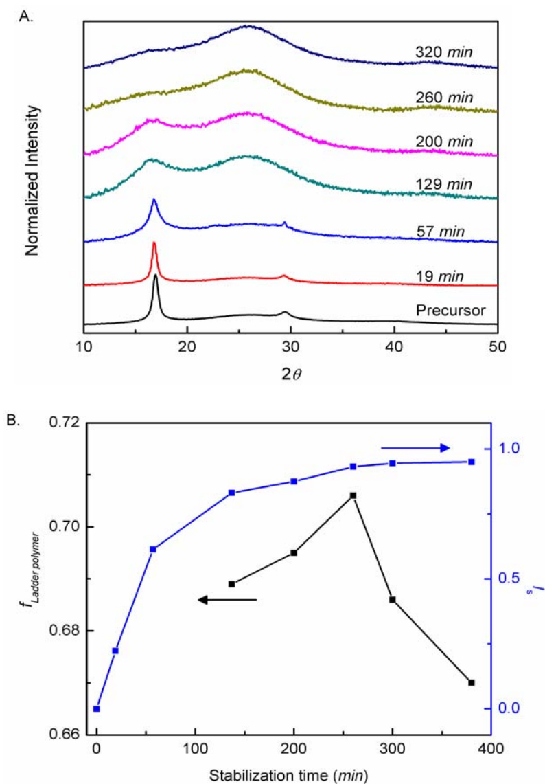
Figure 4. WAXD results of fibers stabilized at 255 °C for various times. (A) Integrated scans and (B) variation of f_{\text{Ladder}} (Herman's orientation factor of stabilized ladder polymer) and I_s (stabilization index) as a function of stabilization time. Intensity profiles of integrated scans in (A) are shifted upward for clear comparison.
