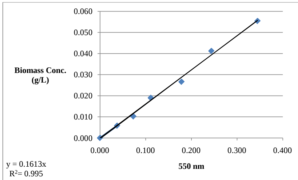
Figure 4.1. Biomass Concentration vs. Absorbance
