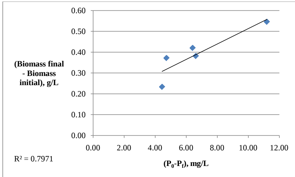
Figure 4.9. Coefficients ( Y_P ) \text{PO}_4\text{-P}
