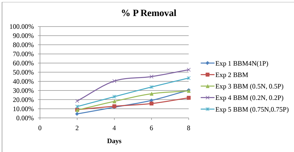
Figure C.19. Effect of media on percent \text{PO}_4\text{-P} removal.
