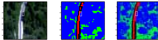
Fig. 3. Left: False RGB composite of a subset of the Urban scene. The 3 \times 2 white rectangle contains a partially occluded section of the road. Middle: Full-pixel classification. The class labels assigned to the pixels inside the rectangle are: road, trees; trees, trees; trees, trees. Note how the road is not complete due to the mixing. Right: Sub-pixel classification. The mixtures obtained in the rectangle are: 0.07 trees + 0.14 trees + 0.78 road, 0.24 trees + 0.46 trees + 0.29 road; 0.42 trees + 0.51 road, 0.81 trees + 0.19 road; 0.46 trees + 0.45 road, 0.85 trees + 0.15 road. Color is assigned by averaging the nonzero coefficients from each class. (This is a color figure.)
