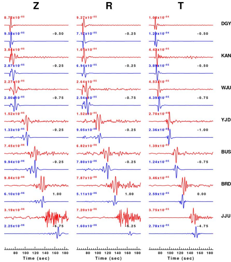
Figure 3. Selected accelerometer recordings integrated to round velocity ( m/s ) and filtered with the sac/gsac commands hp c 0.05 n 3 and lp c 0.20 n 3 . The epicentral distances in km to the stations are DGY (7), KAN (27), WJU (58), YJD (192), BUS (275), BRD (350) and JJU (506). The trace display is discussed in Figure 2.
