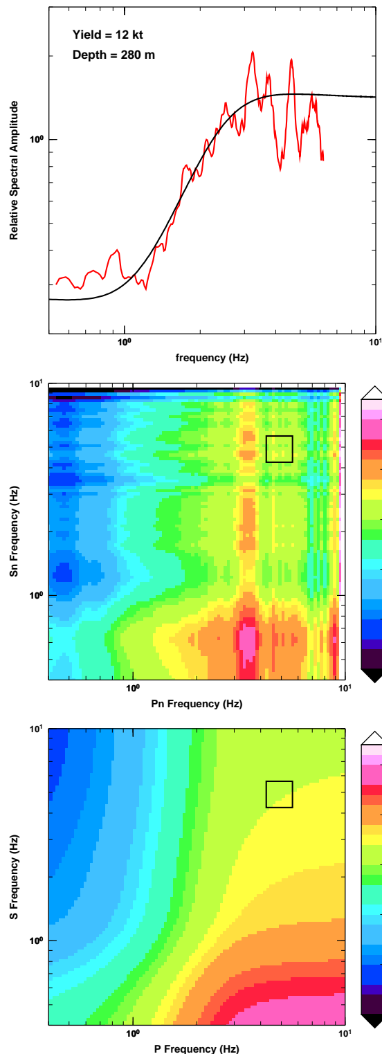
Figure 6. Comparison of model and empirical 1D (top) and 2D (lower two plots) Pn/Sn spectral ratios for the 1998/05/11 UNE in India, using data from station NIL (Nilore, Pakistan).
