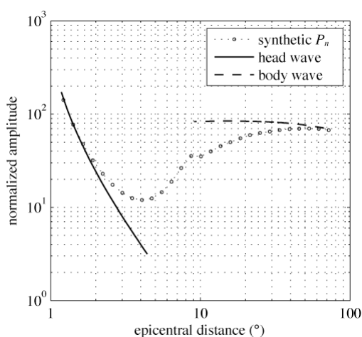
Figure 5. 10-Hz synthetic P_n amplitude decay in a spherical Earth model with constant mantle velocities. The solid line depicts the theoretical amplitude decay of a conical head wave in a plane one-layer-over-half-space Earth model. The dashed line is the amplitude decay of infinite-frequency direct wave in a spherical homogeneous Earth model from ray-tracing calculations.
