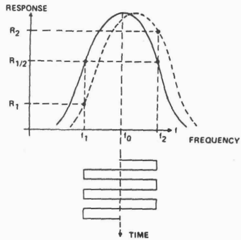
Fig 7 concept for cavity frequency stabilization servo system
