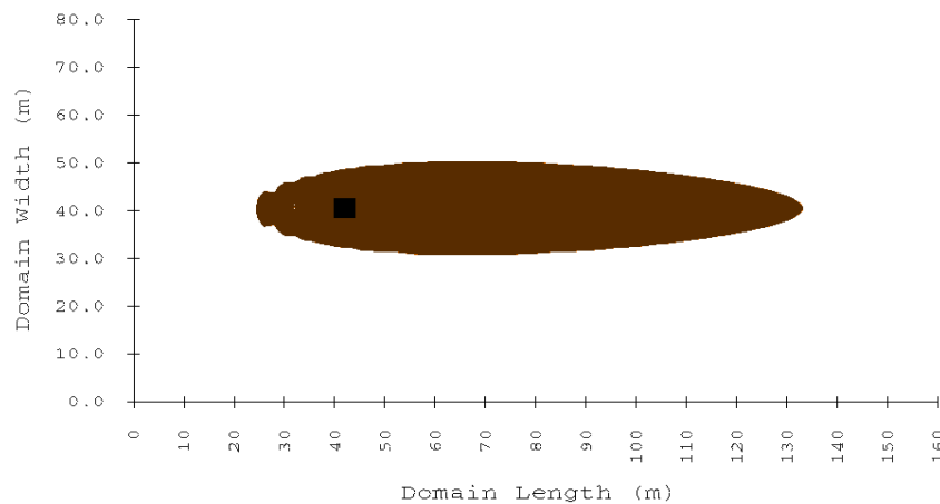
Figure 4-6: Benzene plume 0.005 mg/L contour after 30 years (Scenario B). Model includes sulfate reduction.
