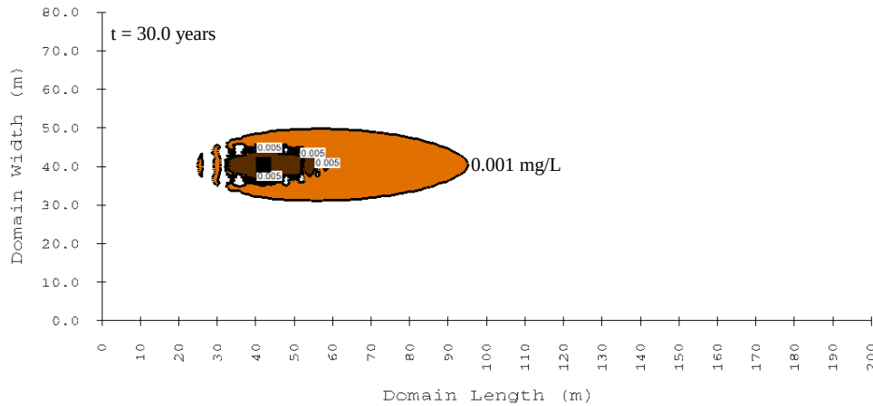
Figure 4-27: Steady-state methanogens concentration ( X_6 ) contours at 30 years ( b_{Met} = 0.00045/d )
