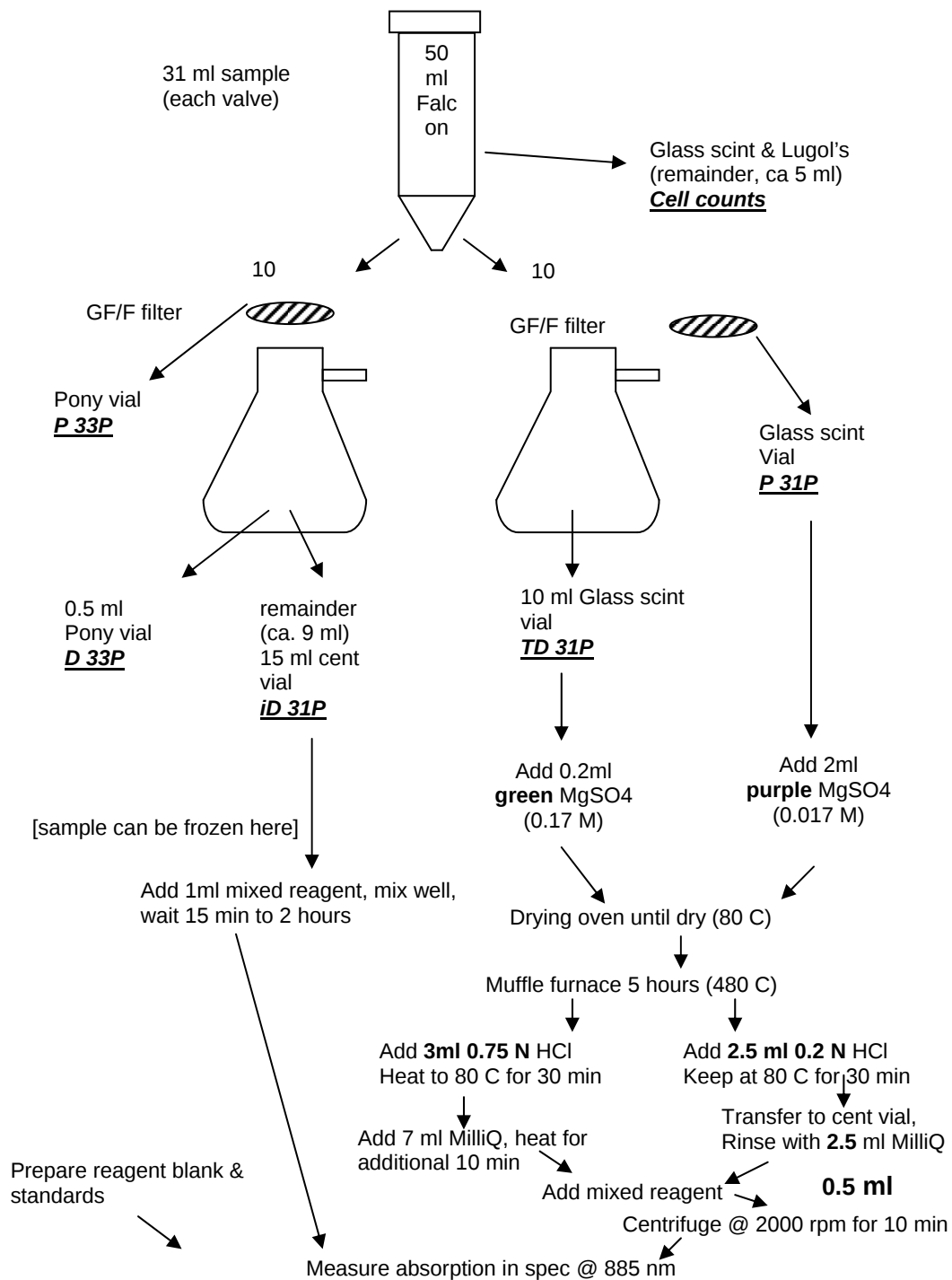
Figure 2. Flow chart illustrating the sample processing procedures to fractionate dissolved and particulate phosphorous, and further measure inorganic dissolved/particulate phosphorous and total dissolved/particulate phosphorous concentrations.
