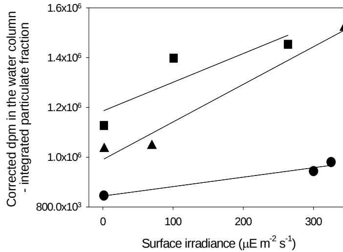
Figure 5. Isotope tracer experiments with the migrating dinoflagellate Akashiwo sanguinea . Water column-integrated incorporation of ^{33}\text{P} into the particulate fraction is dependent on irradiance levels over a 48 hour time course. Circles: experiment 1, triangles: experiment 2, squares: experiment 3. For comparisons, experiments were corrected for radioactive decay of ^{33}\text{P} (half life of 25.4 days), and for the molar isotope dilution of ^{33}\text{P} in the ^{31}\text{P} medium. Experiments differed in cell concentrations of A. sanguinea which is reflected in the elevations of the regression lines.
