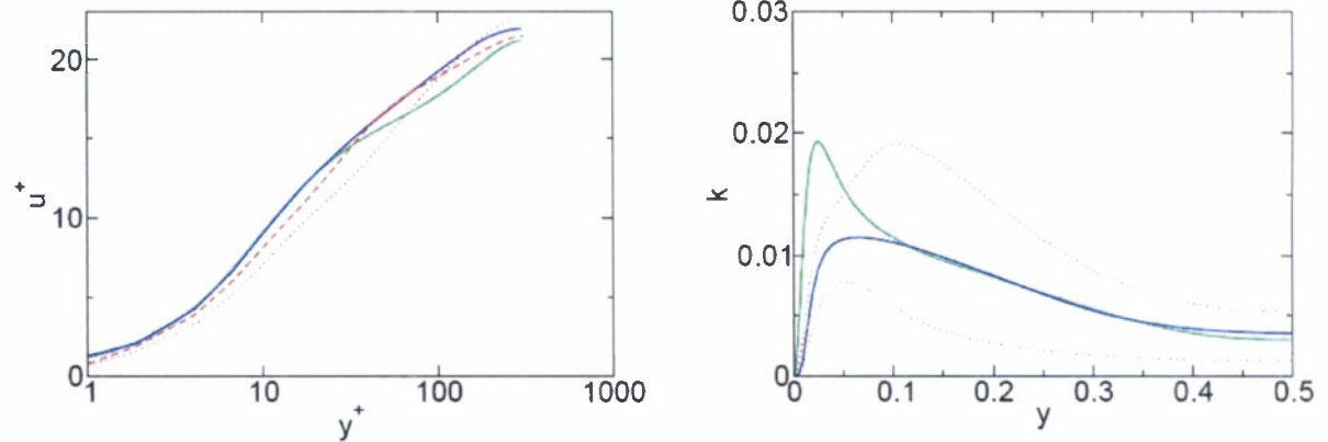
Fig. 6.17: Square-duct flow at Re=10,000 . Wall bisector profiles of a) streamwise velocity in wall units and b) total (red), resolved (orange) and unresolved (magenta) turbulence kinetic energy obtained from FSM simulations . Green lines: DNS; Cyan lines: RANS, 1988 k-\omega low-Re and EASM; Blue lines: RANS, 1998 k-\omega and EASM. Red lines: hybrid models as indicated. Dotted lines: Coarse grid; Dashed lines: Medium grid; Solid lines: Fine grid.
