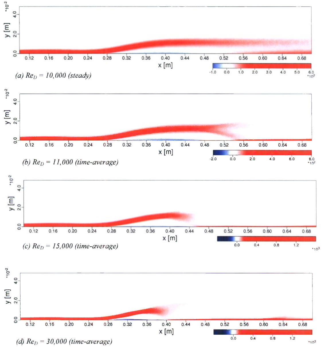
Fig 4.10: Comparison of spanwise vorticity in the mid-span plane for steady and unsteady separation (for the latter obtained from the time-averaged flow data; red - counter-clockwise rotation, blue - clockwise rotation).
