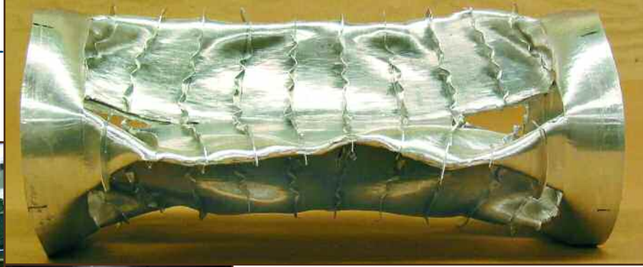
Above: Implosion model after testing. Photo courtesy of R. Kent Tacey, NSWCCD Carderock Division.
