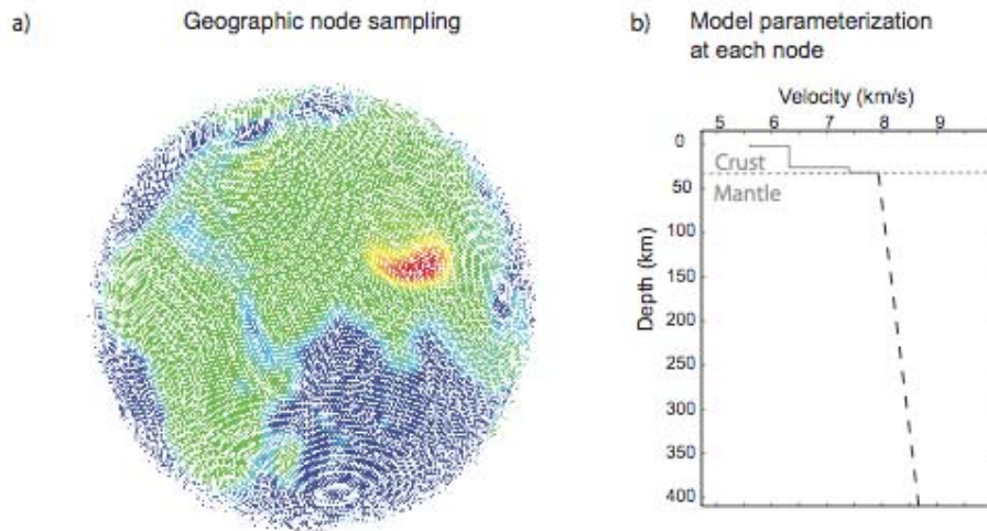
Figure 1. SLBM global parameterization. a) An example tessellation with approximately 1^\circ grid spacing. Color is based on approximate Moho depth. b) An example velocity/depth profile as defined at each node. The mantle portion of the profile is specified by the velocity at the crust/mantle interface and a linear gradient.
