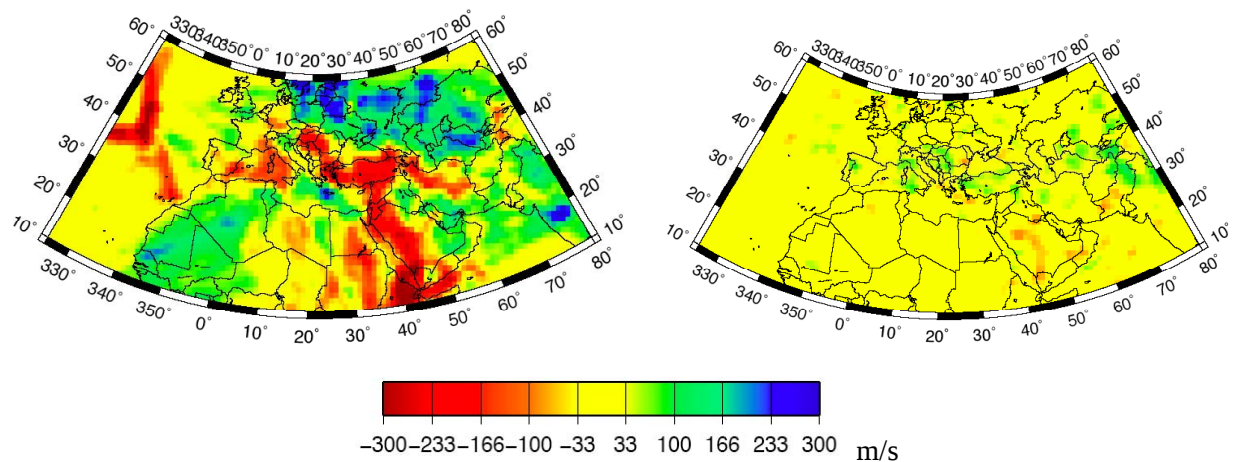
Figure 8. S-velocity perturbations relative to 1-D model MEAN (Marone et al., 2004) at a depth of 100 km (left) and 700 km (right) from our joint inversion.
