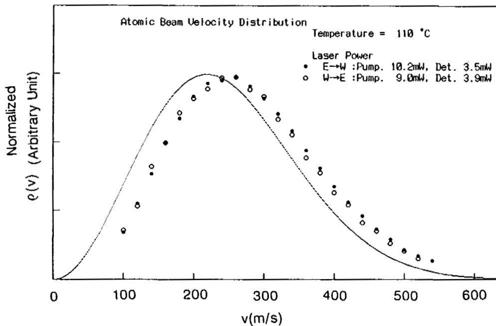
Fig.2 Typical velocity distributions of the optically pumped Cs standard at the NRLM. The solid curve is the calculated Maxwellian distribution.
