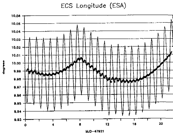
Fig. 7 - ECS 5 longitude from ESA - February 1990 (+ averaged values).
