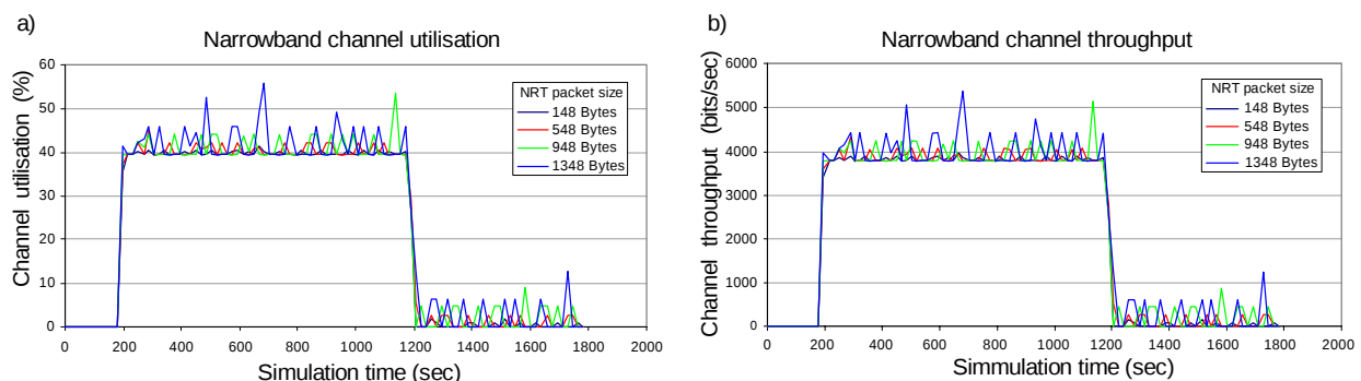
Figure 12. Impact of the NRT packets size onto the narrowband channel utilisation (a) and throughput (b)
