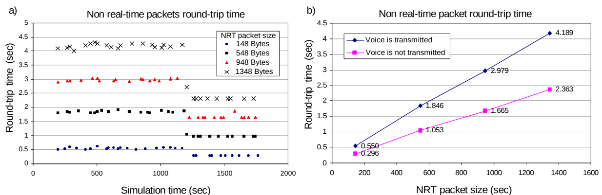
Figure 9. Non real-time packets round-trip time (versus simulation time (a) and versus NRT packets size (b))
