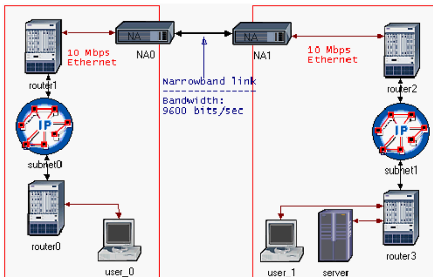
Figure 15. Simulation scenario – extended network
