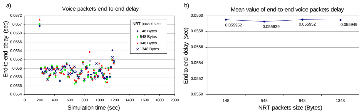
Figure 10. Voice packets end-to-end delay (NRT packets are sent during voice transmission)
