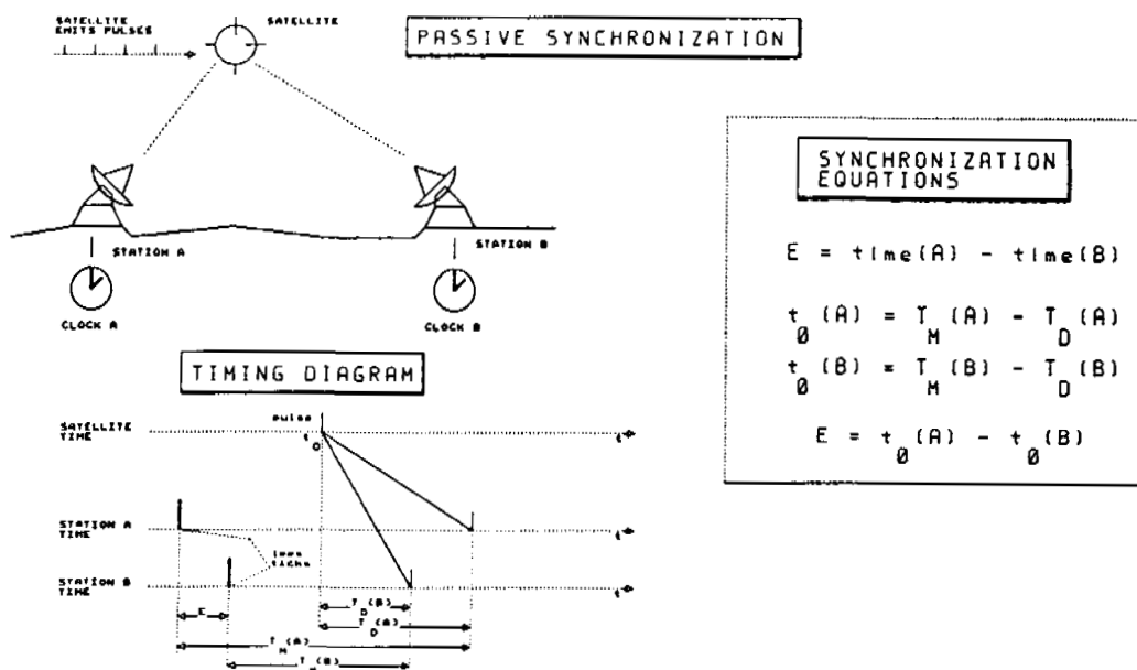
Fig. 2 - PASSIVE SYNCHRONIZATION
