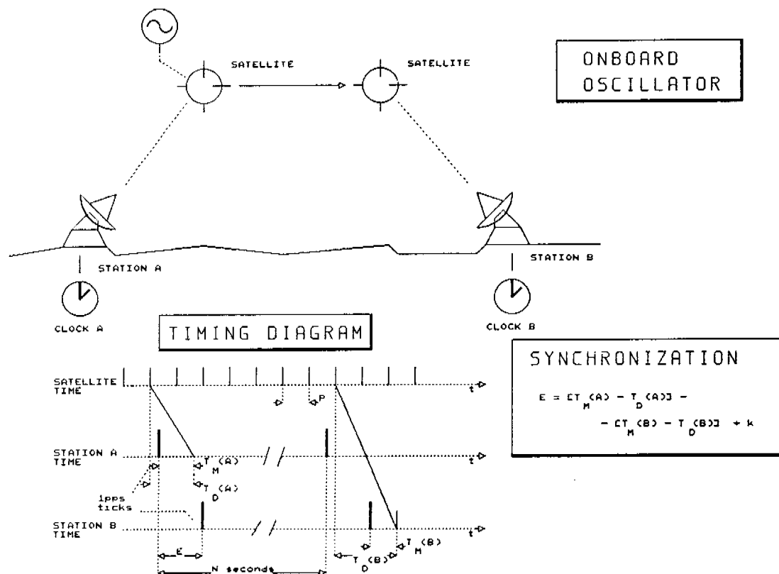
Fig. 3 - SYNCHRONIZATION WITH ORBITING OSCILLATOR
