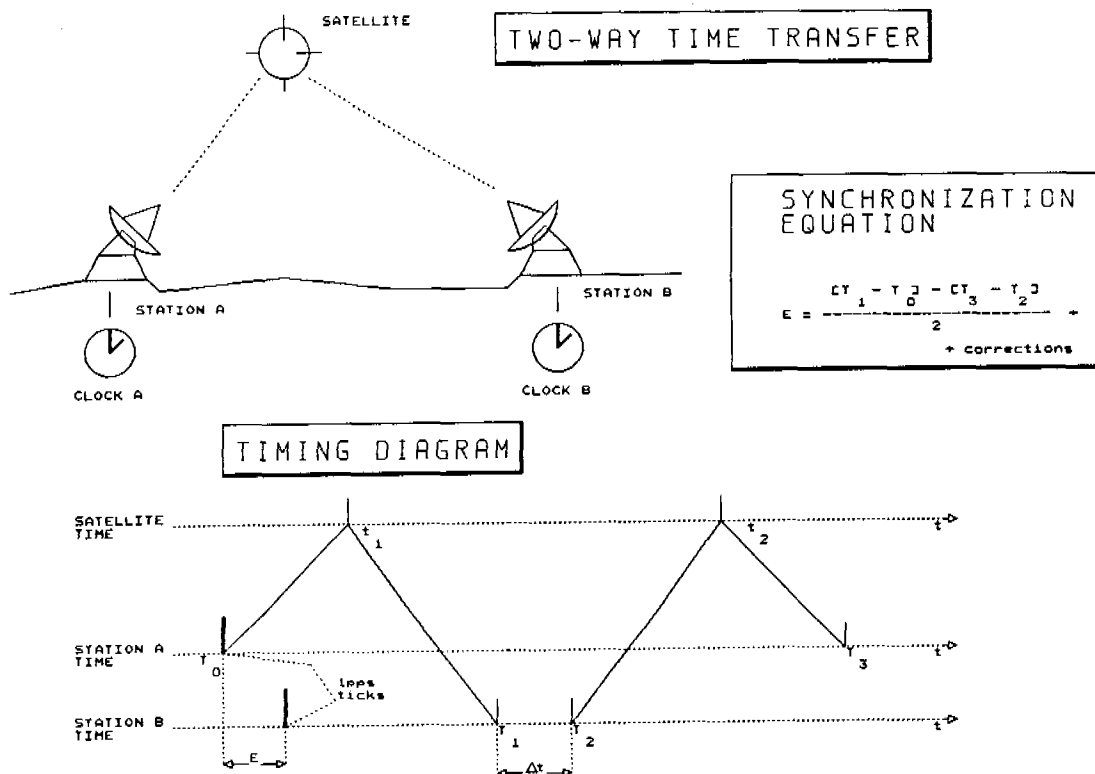
Fig. 5 - TWO-WAY SYNCHRONIZATION
