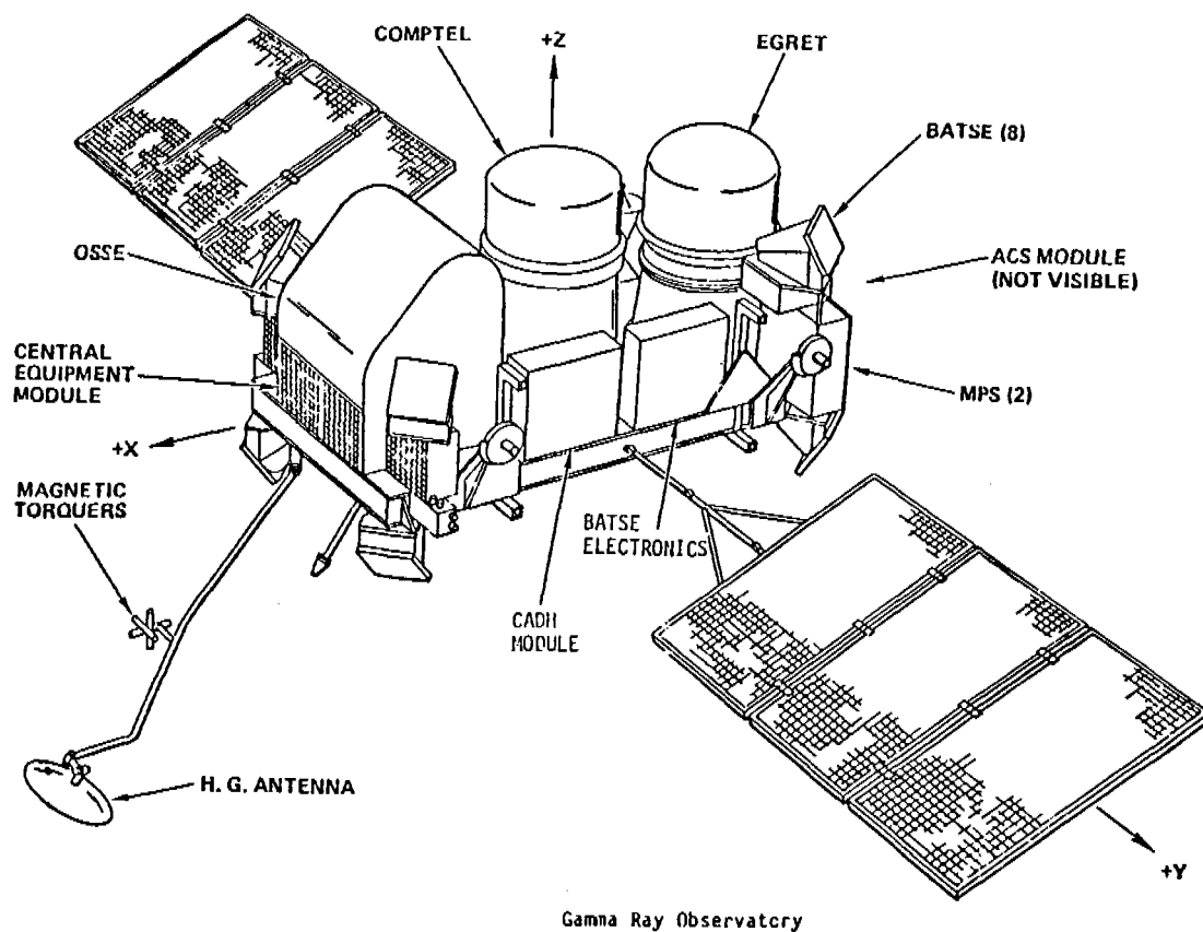
Fig. 13 - The Gamma Ray Observatory (GRO)
