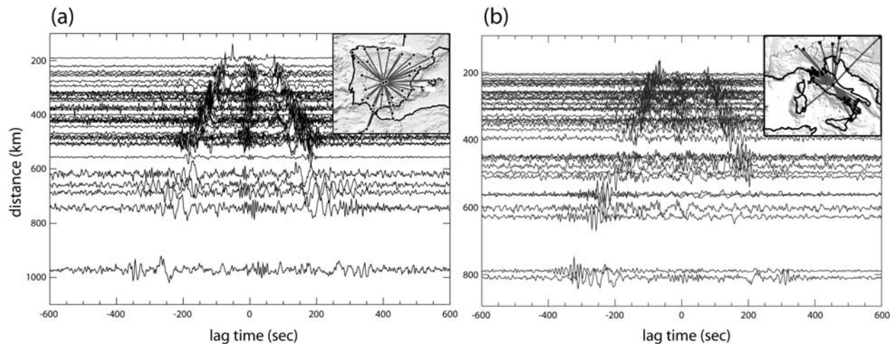
Figure 2. Record sections. (a) From the Spanish National Network. Cross-correlations are from 4 months of data. (b) From stations around Italy. Cross-correlations are from one year of data.
