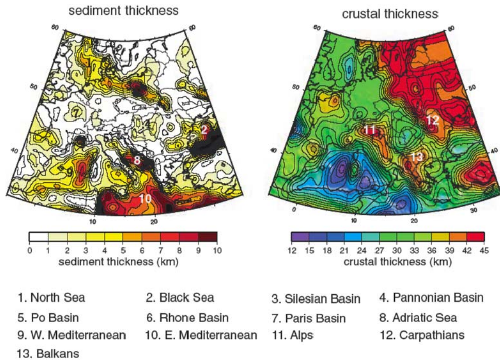
Figure 5. Sediment thickness and crustal thickness presented for comparison with Figure 4. Values taken from CRUST2.0.
