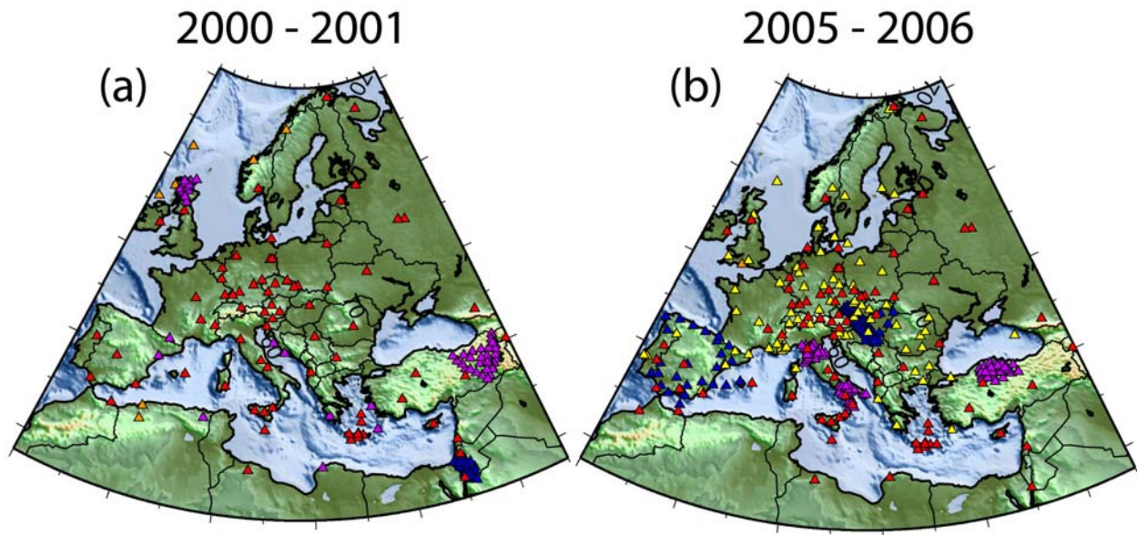
Figure 1. Contrast in station coverage in the years 2000–2001 versus 2005–2006. The station color code is as follows: BLUE—regional networks (e.g., Spanish National Network, the Israeli DESERT2000 experiment); RED—other data available through IRIS; YELLOW—VEBSN data available from the Orfeus Data Center in Europe; PURPLE—PASSCAL experiments or other European PASSCAL-like deployments (such as the MIDSEA experiment); ORANGE—SeisUK stations.
