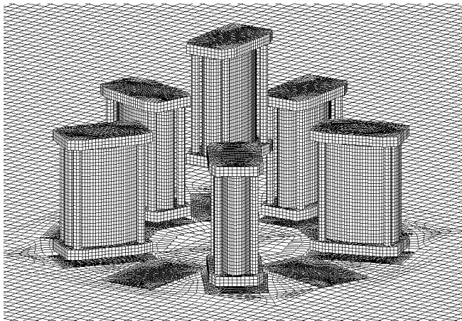
Fig. 5. View of the finite element model showing upper half of array and lower half of 2 \text{ m} \times 2 \text{ m} \times 2 \text{ m} water cube.
