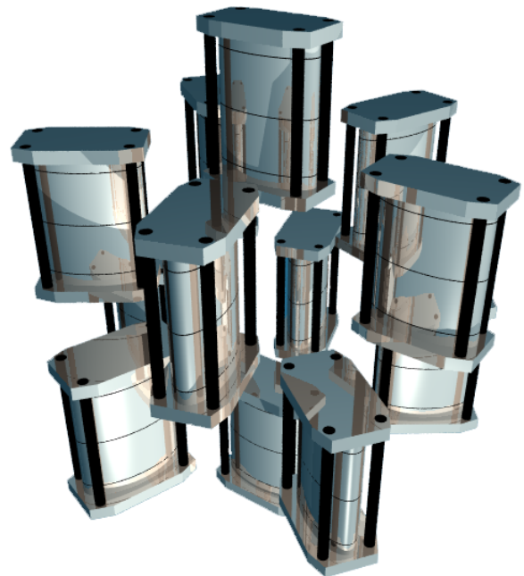
Fig. 1. The icosahedral array of 12 PMN-driven flexensionals (Lockheed Martin and NUWC collaboration).
