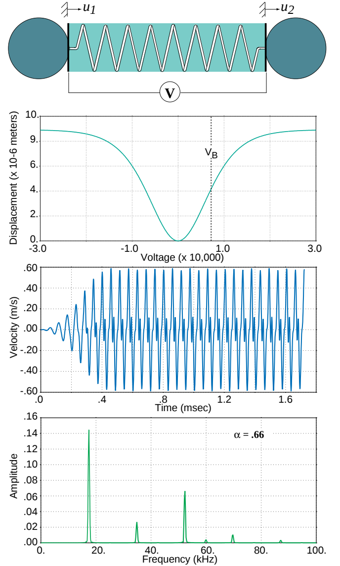
Fig. 2. Nonlinear behavior of the PMN harmonic oscillator model, showing static displacement versus voltage (top), velocity response to a 17.5 kHz sine wave at 66% of the bias voltage V_B (middle) and the spectrum quantifying harmonic generation (bottom).
