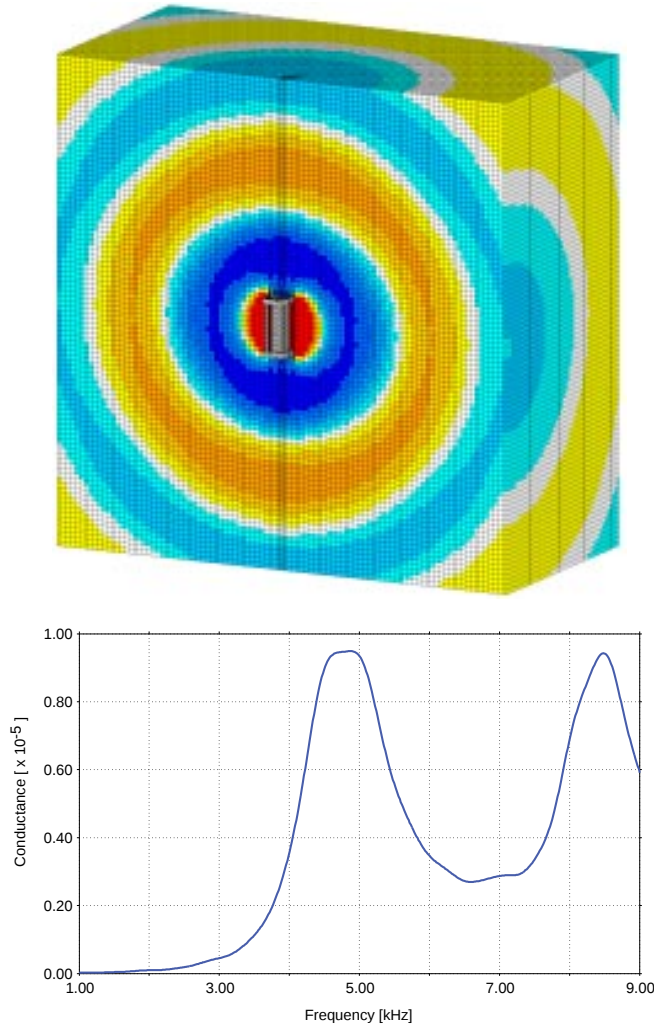
Fig. 3. Behavior of a single flextensional model driven in water, showing wave pattern and electrical response.
