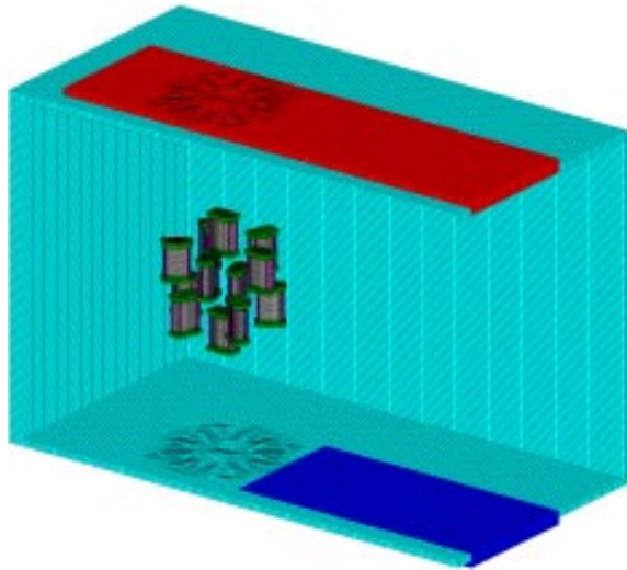
Fig. 7. PZFlex finite element model of icosahedral array within a fiberglass box with steel strongback and lead ballast plate.
