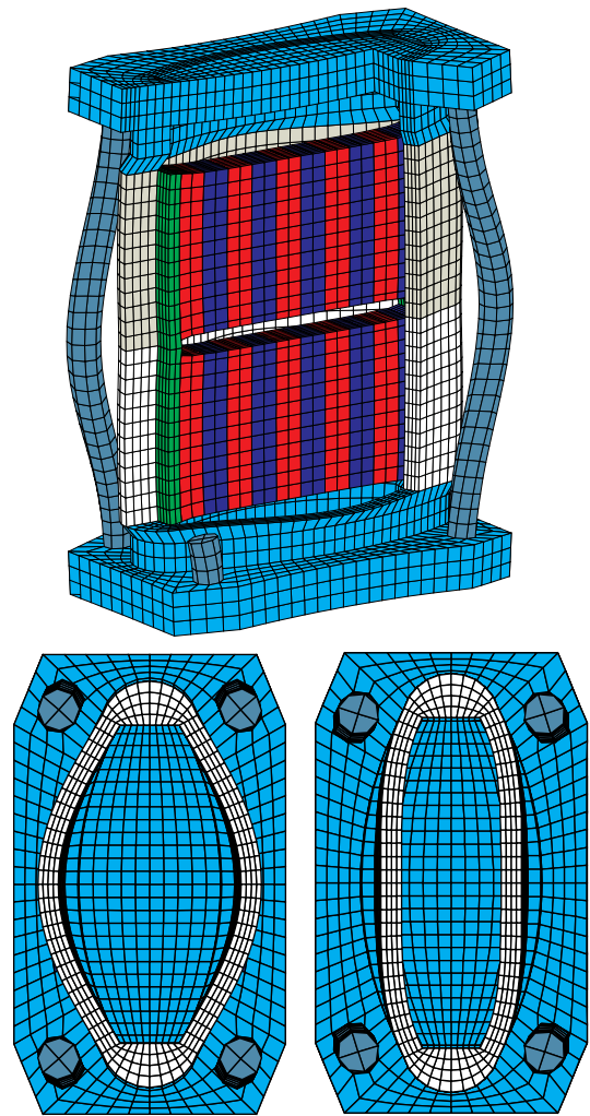
Fig. 4. Views of mode shapes in the single flextensional model driven at 4.5 kHz.
