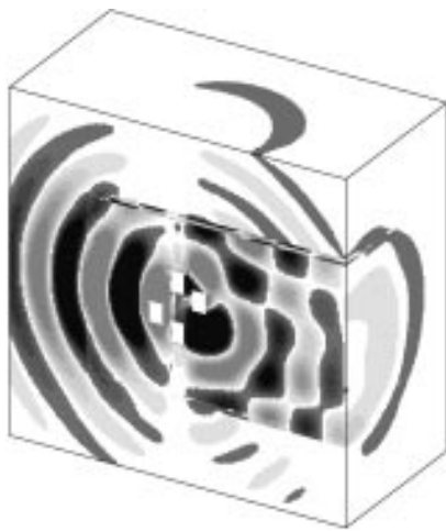
Fig. 8. Radiated acoustic field from the icosahedral array in a fiberglass box with a strongback and ballast plate.
