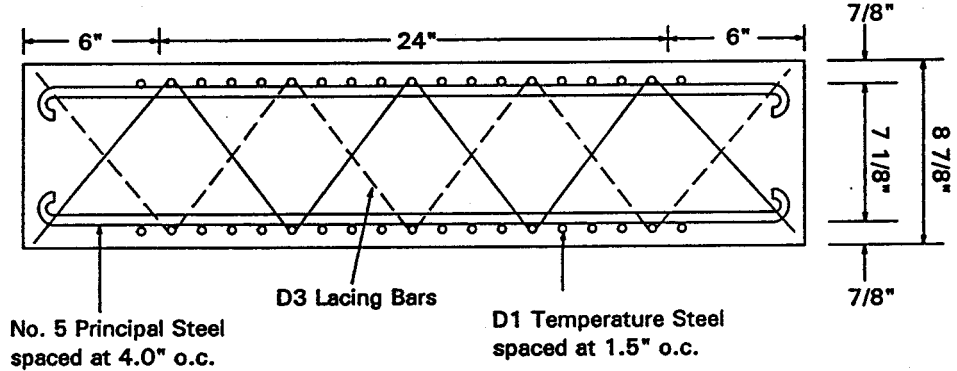
Figure 13. Sectional View Through Length of Slab No. 12
