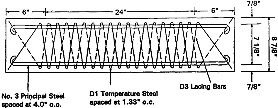
Figure 12. Sectional View Through Length of Slab No. 11
