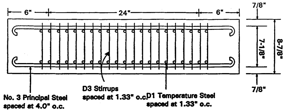
Figure 9. Sectional View Through Length of Slab No. 7
