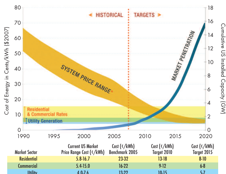
Figure 1. Historic and predicted photovoltaic cost of energy and total installations over time.
