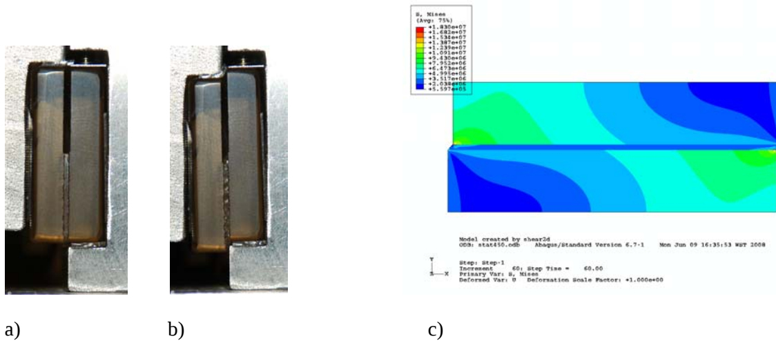
Figure 2 a) and b) show optical images of the specimen during testing. The specimen comprises two glass ceramic plates bonded by a polyurethane layer inbetween. A notch was sawed through the interface (upper section of the specimen) to promote delamination at the interface). Left photograph, a) is under no load, whereas the right photograph, b), is under load (note deformation at the surface of the polyurethane layer between the glass-ceramic plates). c) Finite element model result showing the von-mises stress variation throughout the specimen while under load (orientation of this is inverted and 90 degrees rotated compared with b).
