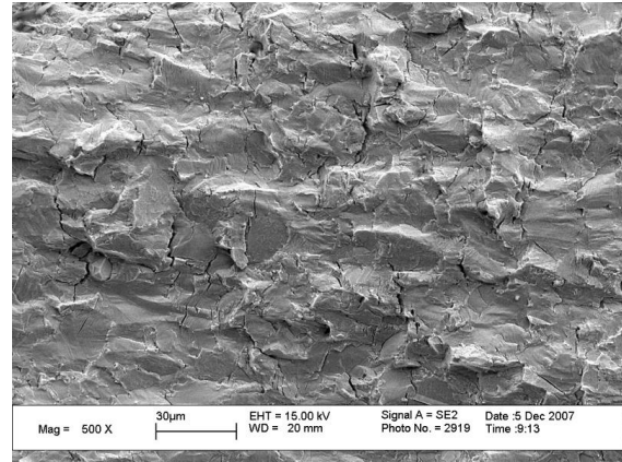
Shear crack (MSS) deflection \theta = 18^\circ
