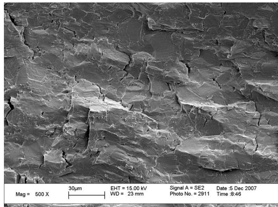
Shear crack (MSS) deflection \theta = 1^\circ
