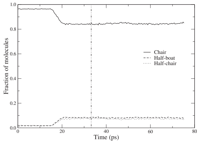
FIG. 11. Fraction of molecules in a given ring conformation after shock loading at U_p = 0.63 \text{ km s}^{-1} . The vertical line denotes the time at which SFABCs were applied.
