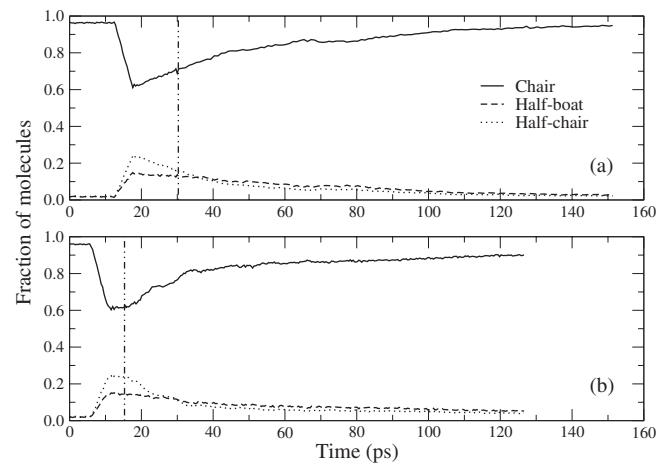
FIG. 12. Fraction of molecules in a given ring conformation in a crystalline region after shock loading at U_p = 1.0 \text{ km s}^{-1} . The vertical lines denote the time at which SFABCs were applied. (a) Long cell and (b) short cell.
