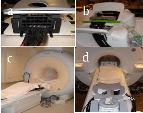
Figure 3: (a) Fiber interface integrated into an Invivo breast coil in a Philips scanner, and (b) a USA Instruments coil in a GE scanner.
