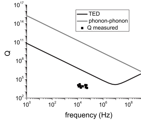
FIG. 8. Solid lines: calculated dissipation in UNCD cantilevers (thickness = 1 \mu\text{m} ) due to TED, phonon-phonon dissipation as a function of frequency. Data points: measured dissipation at fundamental flexural resonance of the cantilevers used in this study. Since diamond remains an ideal Grüneisen's solid independent of the pressure, a Grüneisen's constant of 1 has been used in the models.
