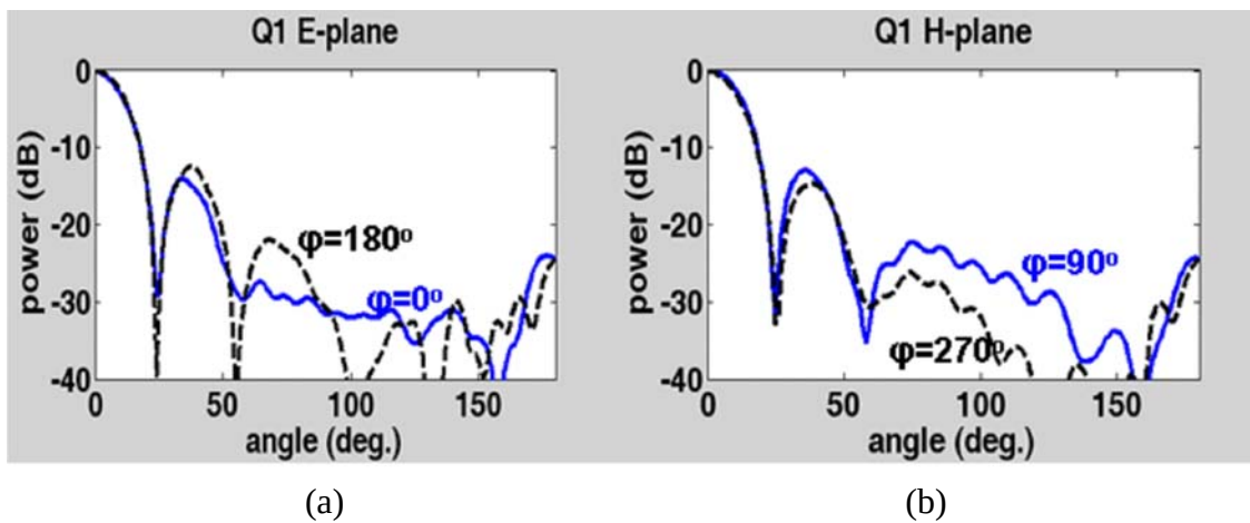
Figure 21. Q1 array pattern at 750 MHz: a) E-plane, and b) H-plane.
