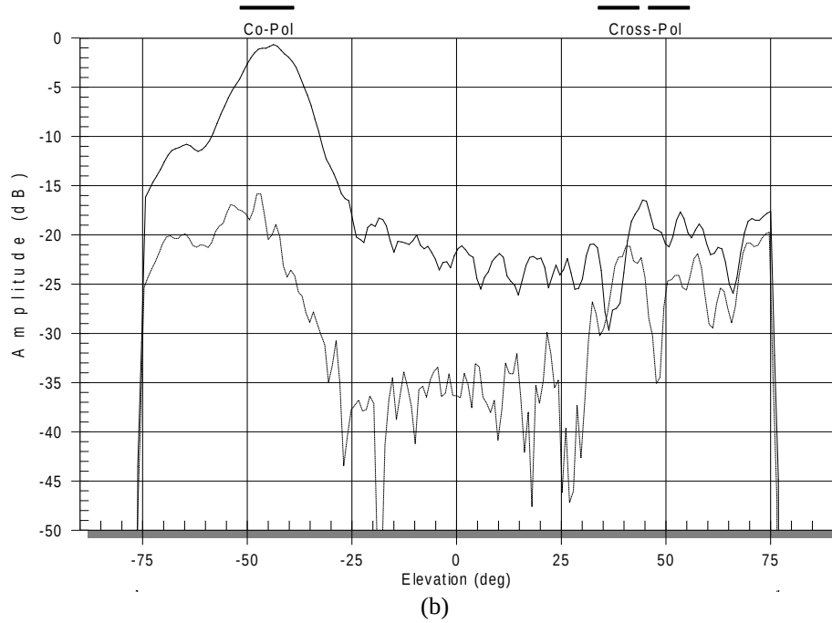
Fig. 11. RHCP Radiation patterns of the 32 radiating SIWs slot array with folded feed networks at 12.45GHz. (a) Azimuth cut. (b) Elevation cut.
