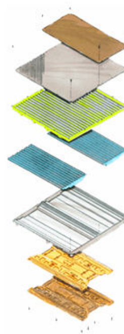
Figure 3.1-1. 38 GHz Point-to-Point CTS Antenna (with Exploded View)
