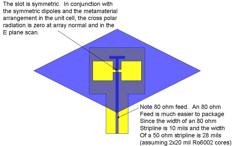
Fig. 3 The 80 ohm stripline feed and the slot in ground plane of the 3D metamaterial wide scan radiating element.
