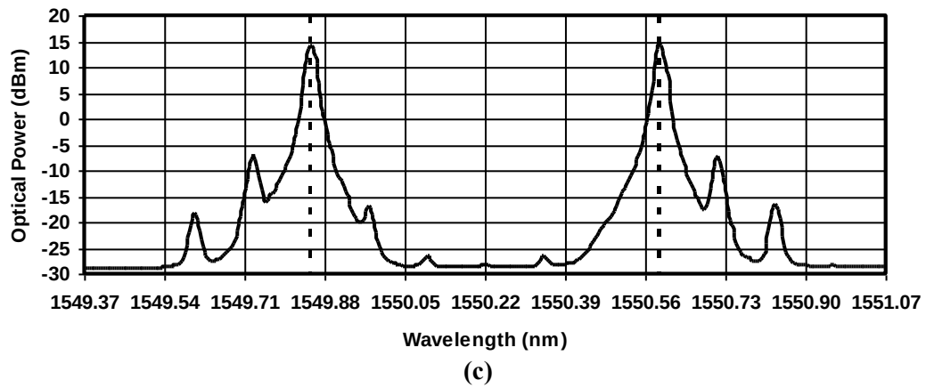
Figure 4: Optical Spectrum Analyzer Output Showing the (a) Spectrum of Sidebands After the First Modulator, (b) Spectrum Of Sidebands After The AWG, (c) Spectrum of the Filtered Sidebands With Data After the EDFA.
