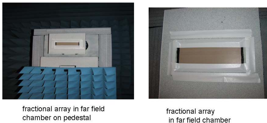
Figure 4 Pictures of the 3D Metamaterial Wide Scan Radiating Element in a Rockwell Collins' Compact Range.
