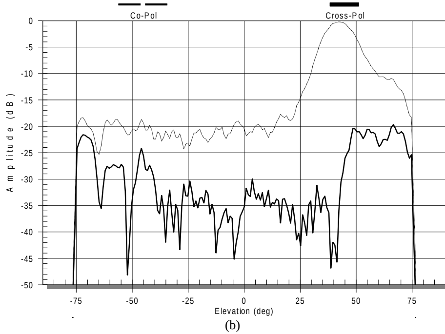
Fig. 10. LHCP Radiation patterns of the 32 radiating SIWs slot array with folded feed networks at 12.45GHz. (a) Azimuth cut. (b) Elevation cut.
