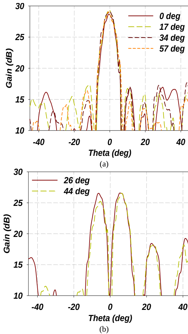
Fig. 21. Measured radiation pattern at inclination angles where the spacing between sub-arrays are multiples of half wavelengths
