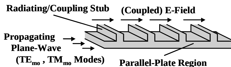
Figure 1.0-1. Basic CTS Radiator /Coupler Configuration (Series-Fed Architecture)
