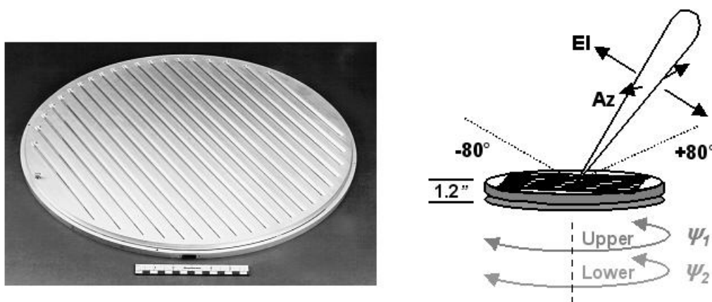
Figure 2.0-1. VICTS Array Scan Geometry
