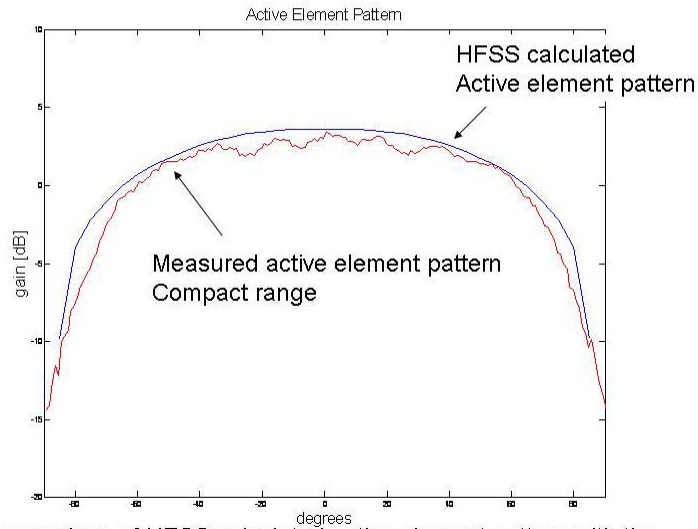
Figure 11 Comparison of HFSS Calculated Active Element Pattern with the Measured Active Element for the E plane at 18 GHz
