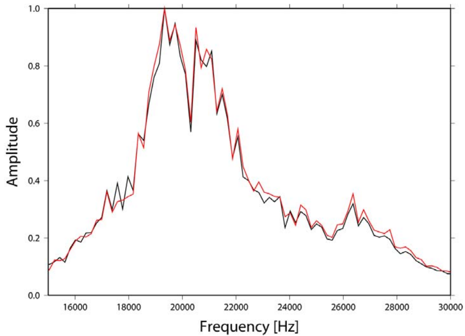
Figure 40: a) Spectrum of the source sweep (same as Figure 24b) b) Superposition of normalized resonance wave amplitude spectra for the proud bomb oriented parallel to the rail (black) and for the proud bomb oriented perpendicular to the rail (red). The resonance waves used to compute the spectra are highlighted by the white rectangles in Figure 39.
