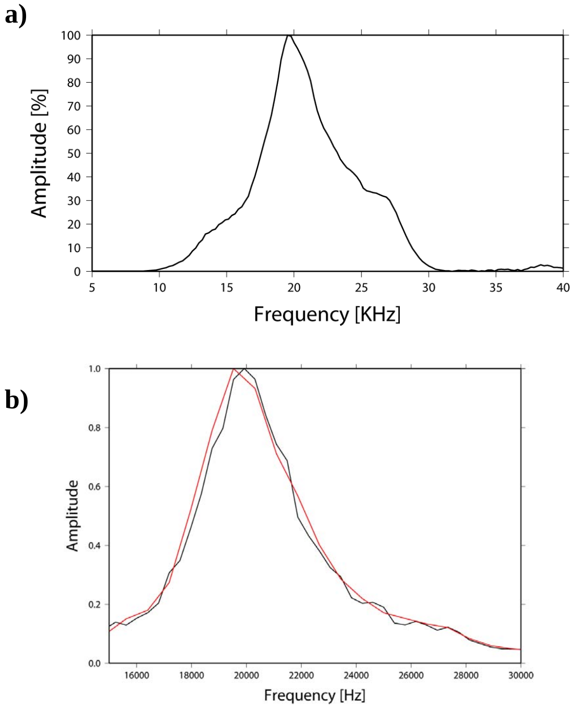
Figure 42: a) Spectrum of the source sweep (same as Figure 24b) b) Superposition of normalized noise spectra for the proud bomb oriented parallel to the rail (black) and for the proud bomb oriented perpendicular to the rail (red). The noise sections used to compute the spectra are highlighted by the white rectangles in Figure 41.
