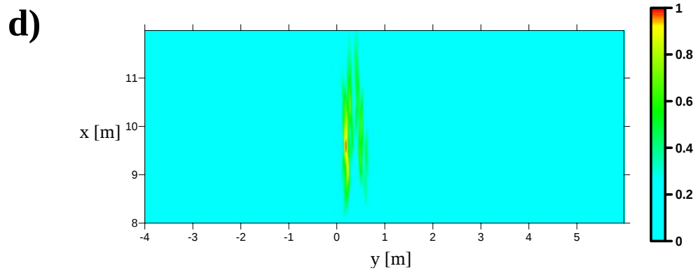
Figure 33 (cont.): d) Two-dimensional plane view of the resonance migrated proud shell using 26,900 Hz data.
