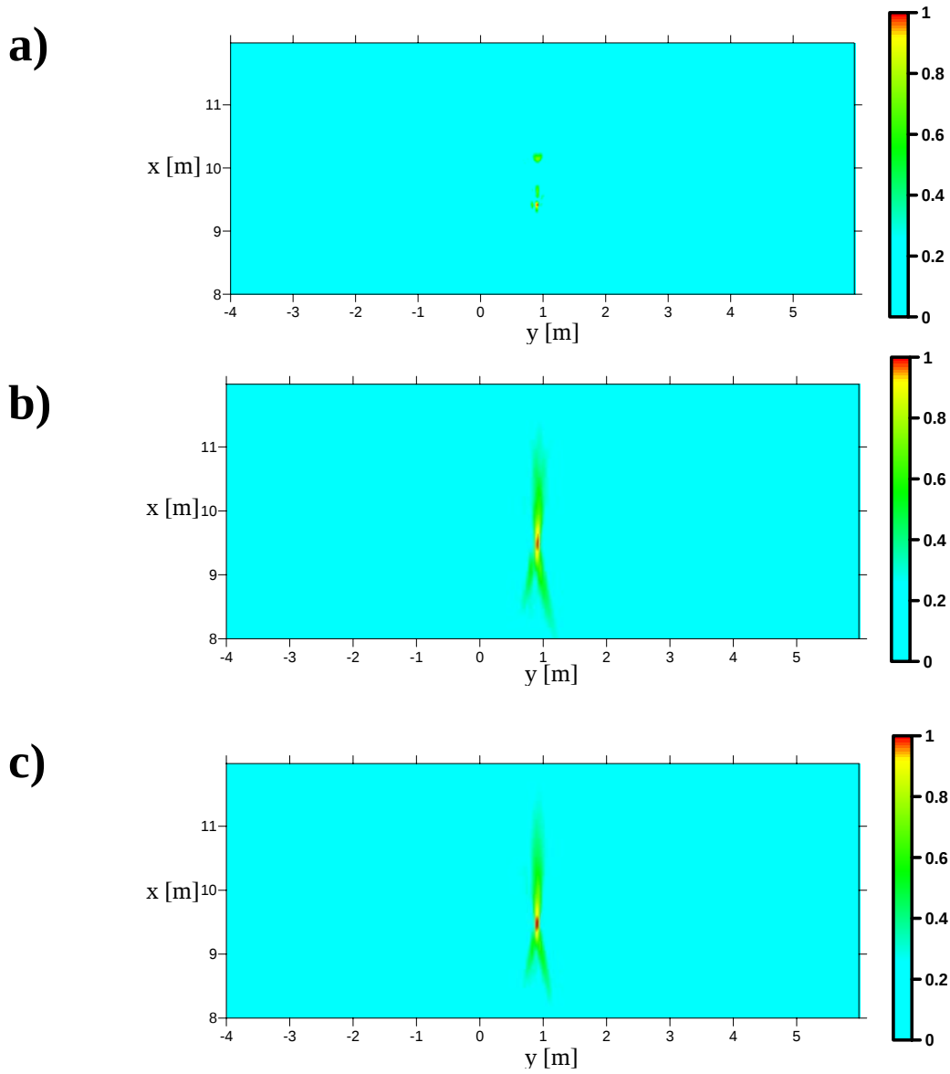
Figure 27: a) Two-dimensional plane view of the Kirchhoff migrated proud sphere using data shown in Figure 25a. b) Two-dimensional plane view of the resonance migrated proud sphere using 12,600 Hz data shown in Figure 26a. c) Two-dimensional plane view of the resonance migrated proud sphere using 16,000 Hz data shown in Figure 26b.
