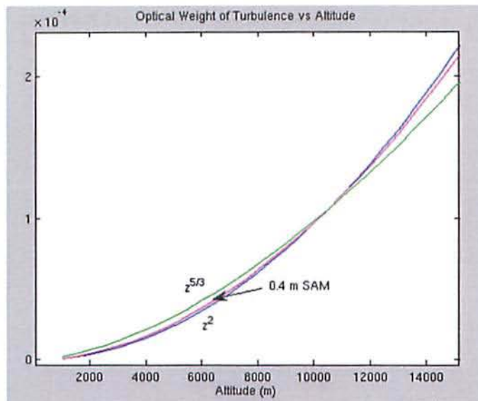
Fig. 6. C_N^2 weights with altitude for SAM and \theta_0
