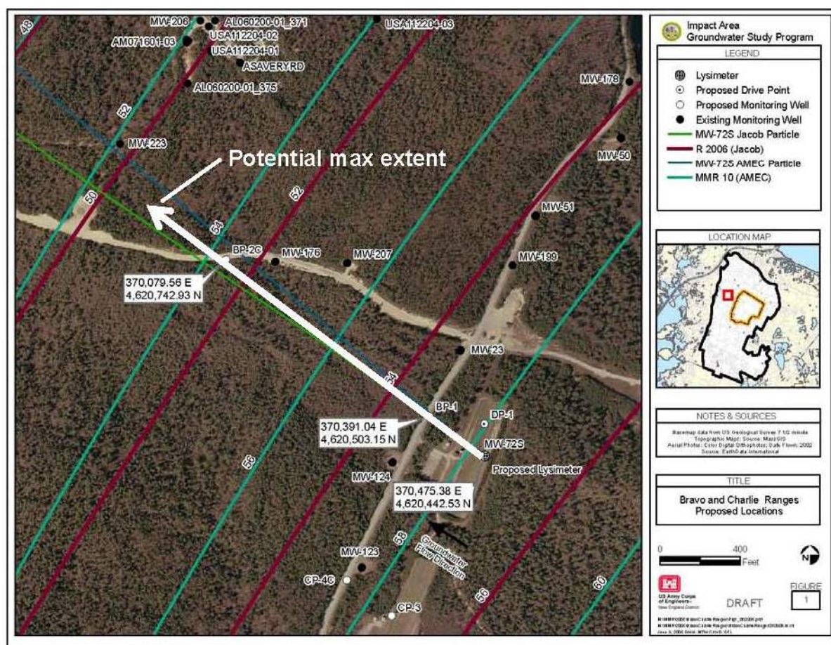
Figure 19. Particle track originating at Bravo Range.
