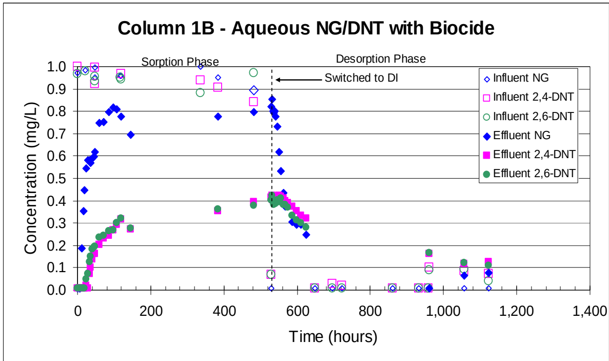
Figure 20. NG and DNT results for column 1B with biocide.
