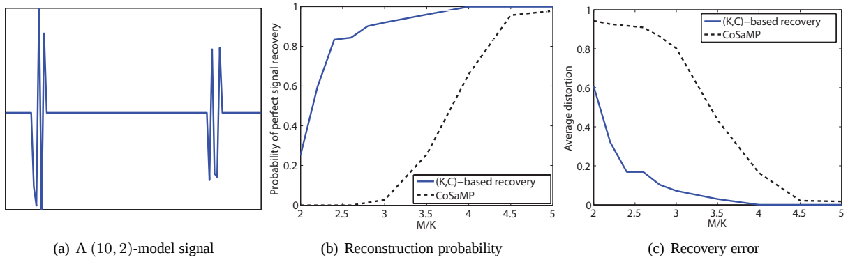
Figure 1: Monte Carlo simulation results for (K, C) -model based recovery with K = 10, C = 2 .
