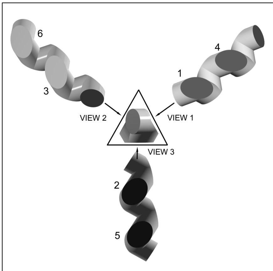
Fig. 2. The triangular tunnel-trap detector where the last three detectors of the generic arrangement are rotated by 180^\circ .
