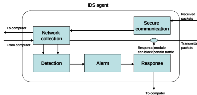
Figure 1: IDS agent
