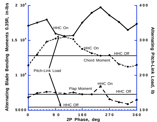
Fig. 4. Variation of alternating blade bending moments and pitch-link load with 2P HHC phase, 1.4 deg amplitude. \mu = 0.15 , C_T/\sigma = 0.09 , \alpha = 3 deg aft.
