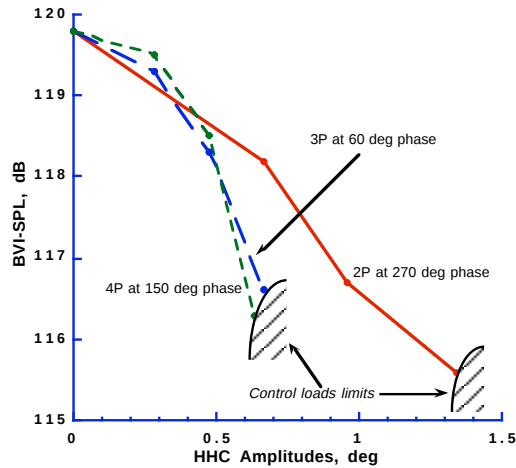
Fig. 6. Variation of BVI noise with HHC amplitude at phases of best noise reduction. \mu = 0.17 , C_T/\sigma = 0.09 , \alpha = 3 deg aft.
