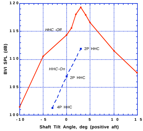
Fig. 8. BVI noise reduction with HHC at different rotor shaft angles. \mu = 0.15 , C_T/\sigma = 0.09 .
