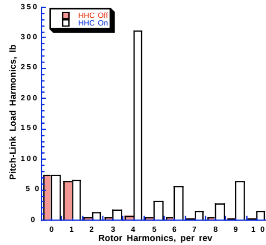
Fig. 11. Effect of 4P HHC for noise reduction on harmonics of pitch-link load. \mu = 0.15 , C_T/\sigma = 0.09 , \alpha = 3 deg forward.
