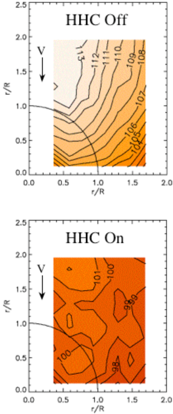
Fig. 9. Noise reduction with 4P HHC over BVI-SPL contour. \mu = 0.15 , C_T/\sigma = 0.09 , \alpha = 3 deg forward.
