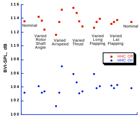
Fig. 12. Effects of trim and flight condition perturbations (increasing left to right) on BVI noise reduction with HHC. Base-line condition: \mu = 0.15 , C_T/\sigma = 0.09 , \alpha = 3 deg forward.
