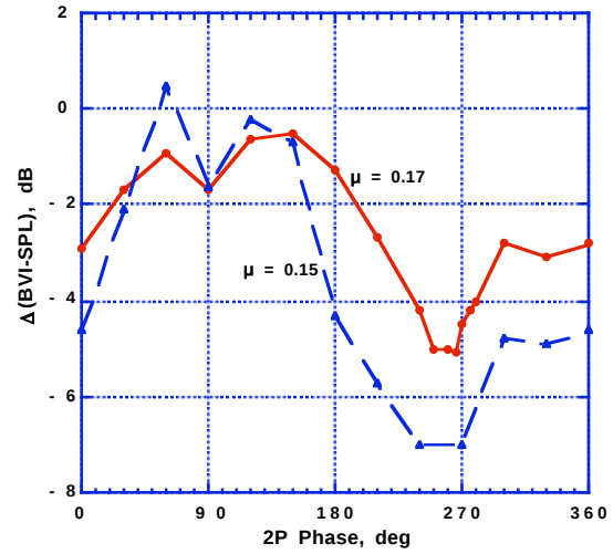
Fig. 7. Variation of BVI noise with 2P HHC phase, 1.4 deg amplitude, at two advance ratios. C_T/\sigma = 0.09 , \alpha = 3 deg aft.
