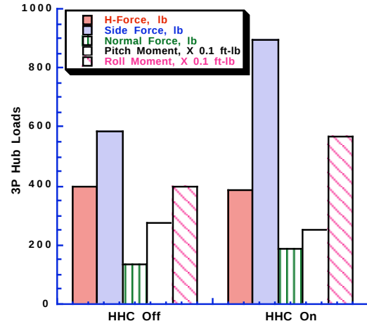
Fig. 10. Effect of 4P HHC for noise reduction on 3P hub loads. \mu = 0.15 , C_T/\sigma = 0.09 , \alpha = 3 deg forward.
