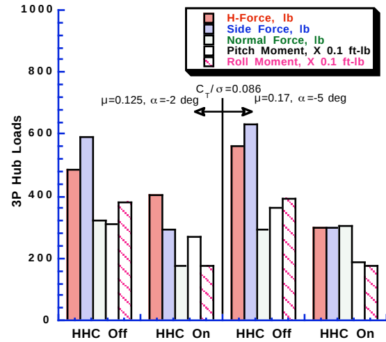
Fig. 14. Reduction in 3P hub loads with the vibration controller at two forward flight conditions.
