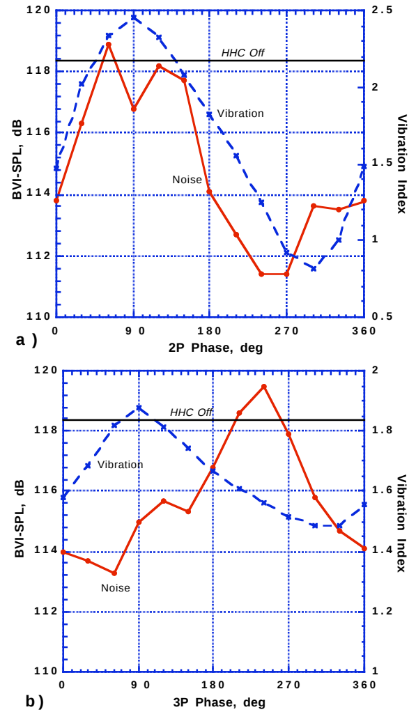
Fig. 3. Variation of BVI noise and 3P hub loads with HHC phase, (a) 2P sweep, 1.4 deg amplitude, (b) 3P sweep, 0.7 deg amplitude. \mu = 0.15 , C_T/\sigma = 0.09 , \alpha = 3 deg aft.
