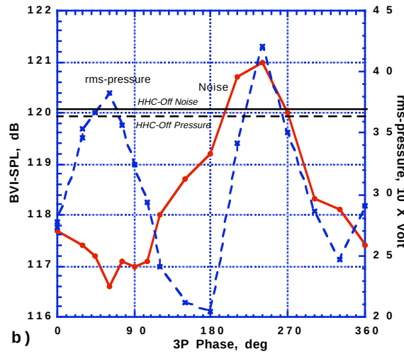
Fig. 5. Variation of BVI noise and rms-pressure signal at 0.85R with HHC phase, (a) 2P HHC, 1.4 deg amplitude, (b) 3P HHC, 0.7 deg amplitude. \mu = 0.17 , C_T/\sigma = 0.09 , \alpha = 3 deg aft.
