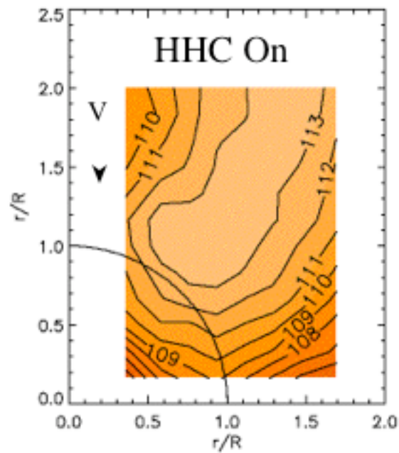
Fig. 13. Noise reduction using noise controller with blade pressure feedback over BVI-SPL contour. \mu = 0.15 , C_T/\sigma = 0.09 , \alpha = 3 deg aft.
