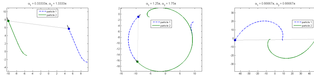
(a) Case I: Rectilinear equilibrium ( \pi/3, 4\pi/3 ) (b) Case III: CW circling equilibrium ( 5\pi/4, 7\pi/4 ) (c) Case VII: CCW “outward sweep” ( 2\pi/3, 2\pi/3 )
