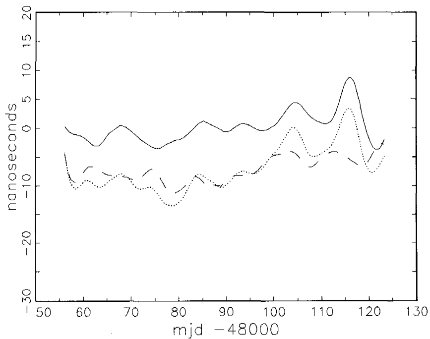
FIGURE 6: Difference between the corrected and the raw values UTC(OP) - UTC(NIST) . The corrected values UTC(OP) - UTC(NIST) are obtained with: — precise ephemerides, --- measured ionospheric delays, ..... precise ephemerides and measured ionospheric delays.
