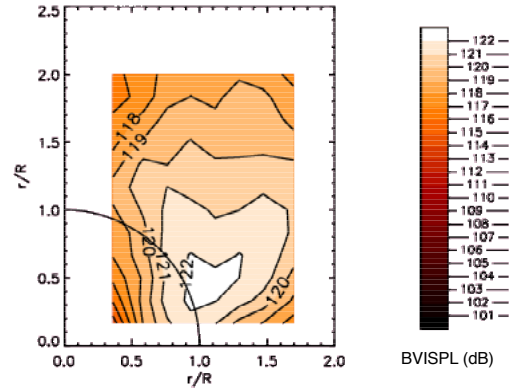
Fig 18. Acoustic footprint of rotor with -2^\circ subwings. M_{tip} = 0.691 , C_T/\sigma = 0.09 , \mu = 0.17 , \alpha_{pp} = 3^\circ .
