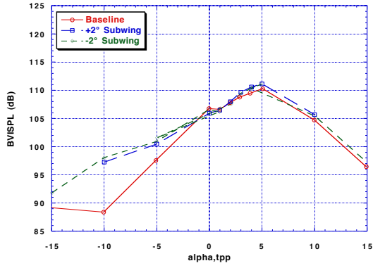
Fig 15. Comparison of two subwings with baseline rotor. M_{tip} = 0.691 , C_T/\sigma = 0.09 , \mu = 0.17 . Mic #9.
