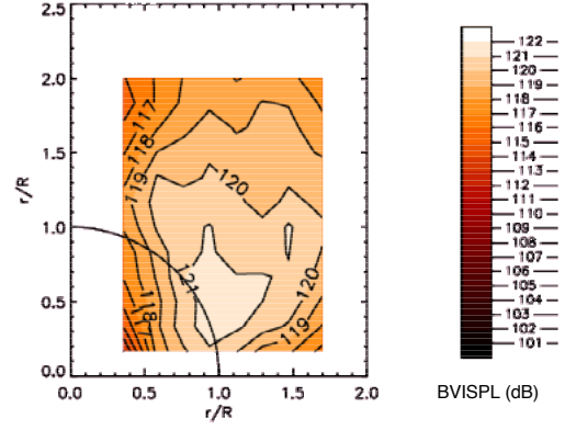
Fig 17. Acoustic footprint of rotor with +2^\circ subwings. M_{tip} = 0.691 , C_T/\sigma = 0.09 , \mu = 0.17 , \alpha_{pp} = 3^\circ .
