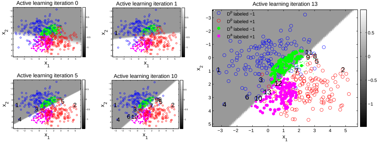
Figure 3: Illustration of active data selection by MigLogit. Only iterations 0,1,5,10,13 are shown. The different symbols are defined as: blue \circ = D^p labeled “-1”, red \circ = D^p labeled “+1”, green \bullet = D^a labeled “-1”, and magenta \bullet = D^a labeled “+1”. The numbers in black denote D_l^p and represent the order of selection. The smaller \bullet near the decision boundaries symbolize weakened participation of the associated D^a in determining w . This may only be visible in the zoomed figure (iteration 13).
