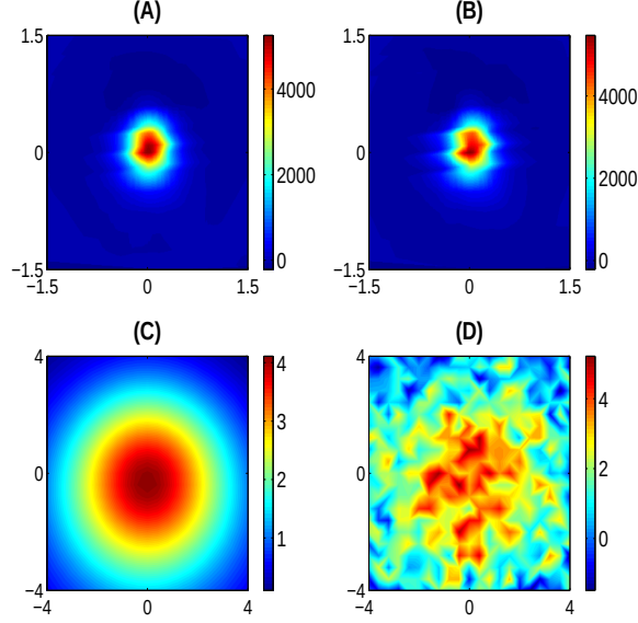
Fig. 2. Process of simulating coarse-resolution (helicopter-based) magnetometer data. (A) Measured fine-resolution (ground-based) magnetometer data. (B) Synthesized fine-resolution (ground-based) magnetometer data using the model parameters obtained from the model inversion with the data in (A). (C) Synthesized noise-free coarse-resolution (helicopter-based) magnetometer data using the model parameters obtained from the model inversion and the data in (A). (D) Same as (C) except with (sensor) noise added.
