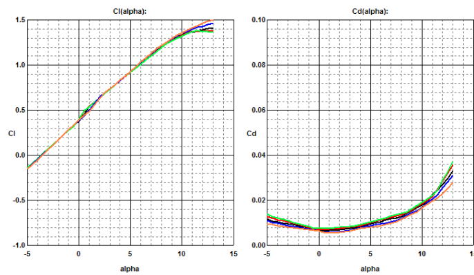
Figure 6.2 Profili2 C_l and C_d versus Alpha Graphs
