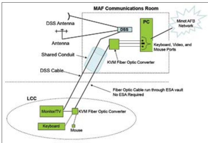
Figure 3. NetLink wiring diagram.
