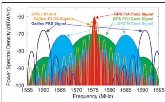
Figure 2. GPS and Galileo Signal Spectra in the Upper L1 band (1555-1595 MHz).
