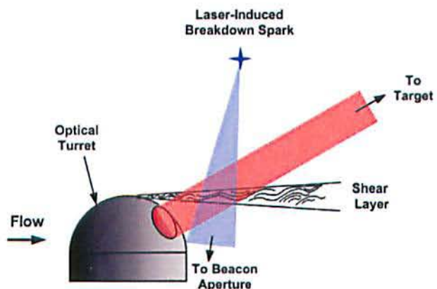
Fig. 1 Conceptual deployment of a laser-spark beacon system.
