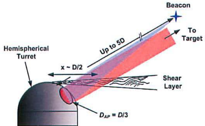
Fig. 9 Possible beacon geometry for a deployed system.
