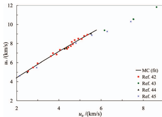
FIG. 7. N_2 Hugoniot in the u_s - u_p plane. Experimental results (filled symbols) are taken from Refs. 42–44; theoretical results were calculated using o - N (MC) 2 (solid line, present work) and AIMD (cross Ref. 45). MC simulations were restricted to the molecular regime (up to P=40 –45 GPa), and have been shifted according to Eq. (42). Here, for ease of viewing, the 28 individual o - N (MC) 2 points results shown explicitly in Fig. 6 were replaced by a quadratic fit after transformation between the P - V and u_s - u_p planes.
