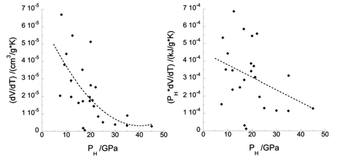
FIG. 4. Partial derivatives of volume with respect to temperature at fixed pressure (left panel), as calculated from results of o -n(MC) 2 simulation performed at the ( P = P_{\text{opt}}, T = T_{\text{opt}} ) combinations shown in Table IV. The right panel shows the same data, but following multiplication by pressure; as described in the text, these pressures are taken to correspond to Hugoniot values ( P = P_H ) by construction. The partial derivative is evaluated using Eq. (44), and the dashed lines represent quadratic (left) and linear (right) fits to the data. Note the difference in ordinate scales.
