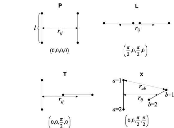
FIG. 1. Diatomic pair configurations used to parametrize the reference potential whose behavior is illustrated in Fig. 2. Bond lengths were held fixed at l=1.117 Å, while c.m. separations r_{ij} were swept over a range of roughly 1.6–6.6 Å, depending on the configuration type (see text). Configuration types are characterized by four angles, (\theta_1, \chi_1, \theta_2, \chi_2) , where \theta and \chi represent rotation of molecules 1 and 2 within and out of the plane of the page. Clockwise rotations are positive, and all angle values are zeroed to those of the P configuration.
