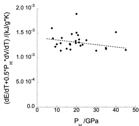
FIG. 5. Evaluation of the denominator appearing in Eq. (42) as calculated from results of o - n (MC) 2 simulation performed at the (P=P_{\text{opt}}, T=T_{\text{opt}}) combinations shown in Table IV. As described in the text, these pressures are taken to correspond to Hugoniot values ( P=P_H ) by construction and the corresponding Hugoniot values for temperature are recovered by use of Eq. (42). The dashed line is a linear fit to the data.
