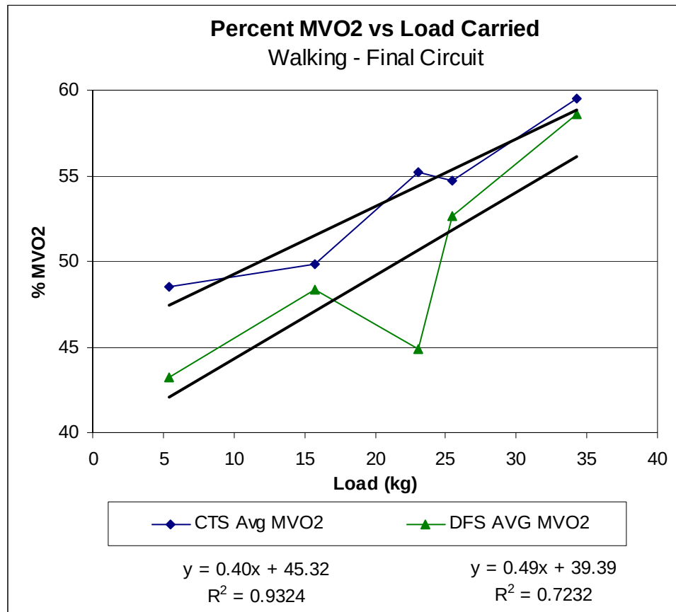
Figure 7: Percent \dot{MVO}_2 versus Load Carried While Walking. CTS refers to the Canadian Cloth the Soldier Pack, DFS refers to the Dynamic Framesheet™.
