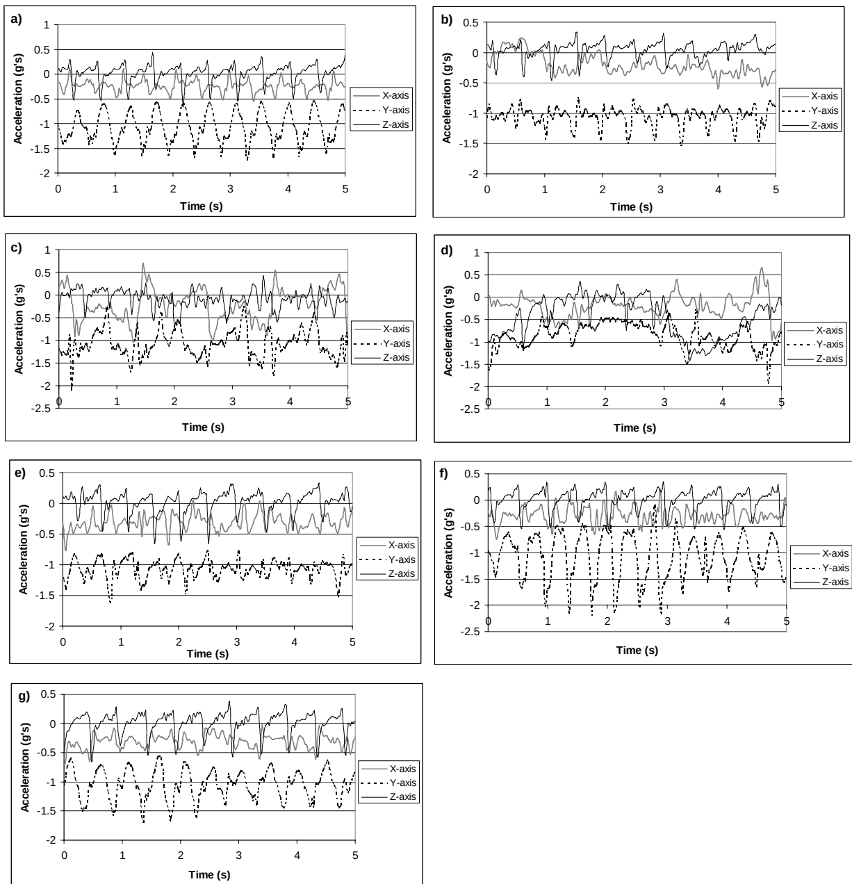
Figure 2: Representative x-, y- and z-axis acceleration patterns for the seven tasks included in the activity circuit (subject: 7MOA, medium load): a) walk; b) balance beam; c) boulder hop; d) over-under barriers; e) slalom run; f) up-down ramp; g) sidehill ramp.
