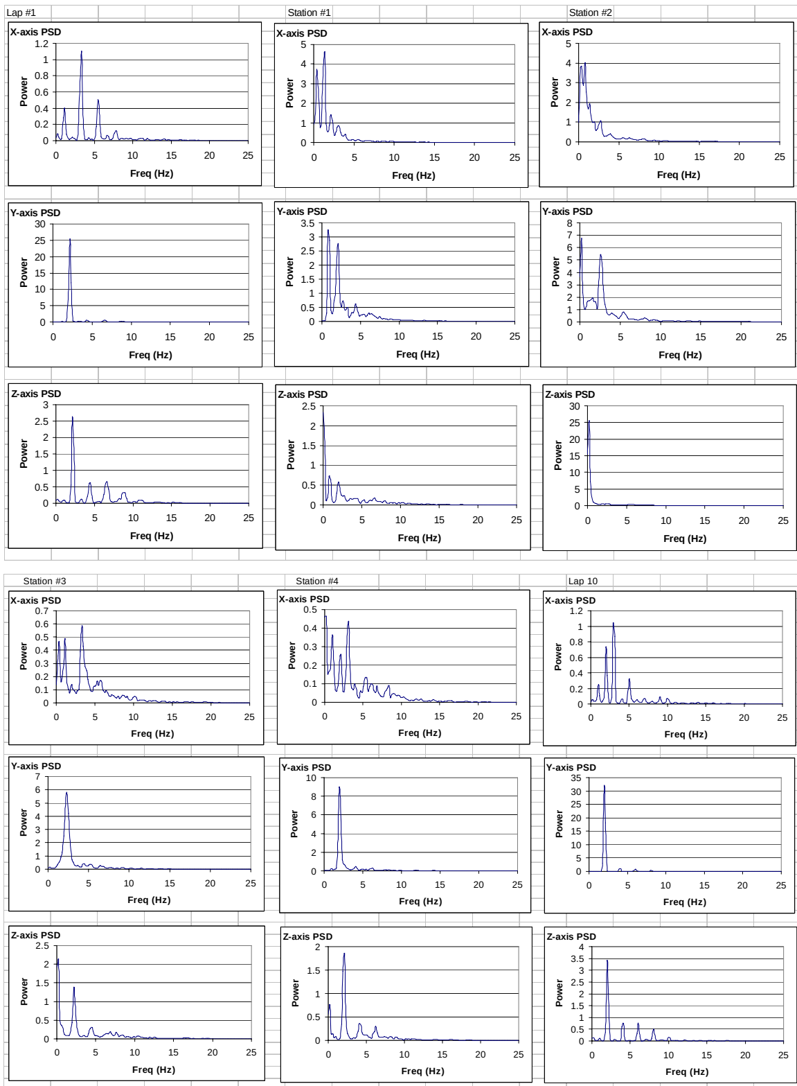
Figure 9: Representative PSD's for lap 1, station 1, station 2, station 3, station 4 and lap 10 from subject 7MOA – medium load. Stations are defined in Table 2.
