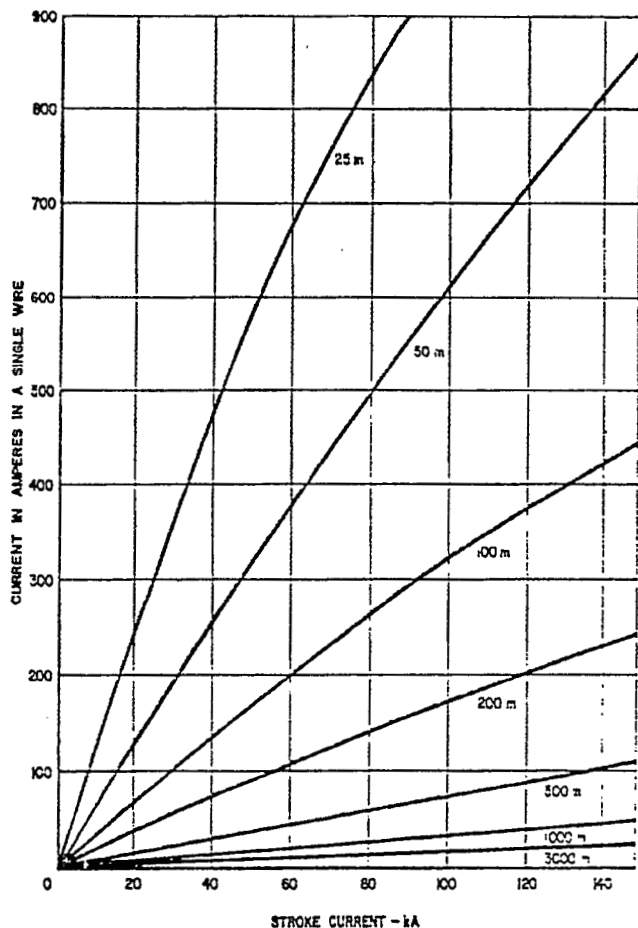
Figure 5. Current to earth at the ends of a single horizontal wire for various crest stroke currents and separating distances (zero soil resistivity).
