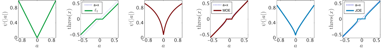
Fig. 3: Left to right: \ell_1 (green), MOE (red) and JOE (blue) regularizers and their corresponding thresholding functions \text{thres}(x) := \arg \min_a \{(x-a)^2 + \lambda \psi(|a|)\} . The unbiasedness of MOE is due to the fact that large coefficients are not shrunk by the thresholding function. Also, although the JOE regularizer is biased, the shrinkage of large coefficients can be much smaller than the one applied to small coefficients.
