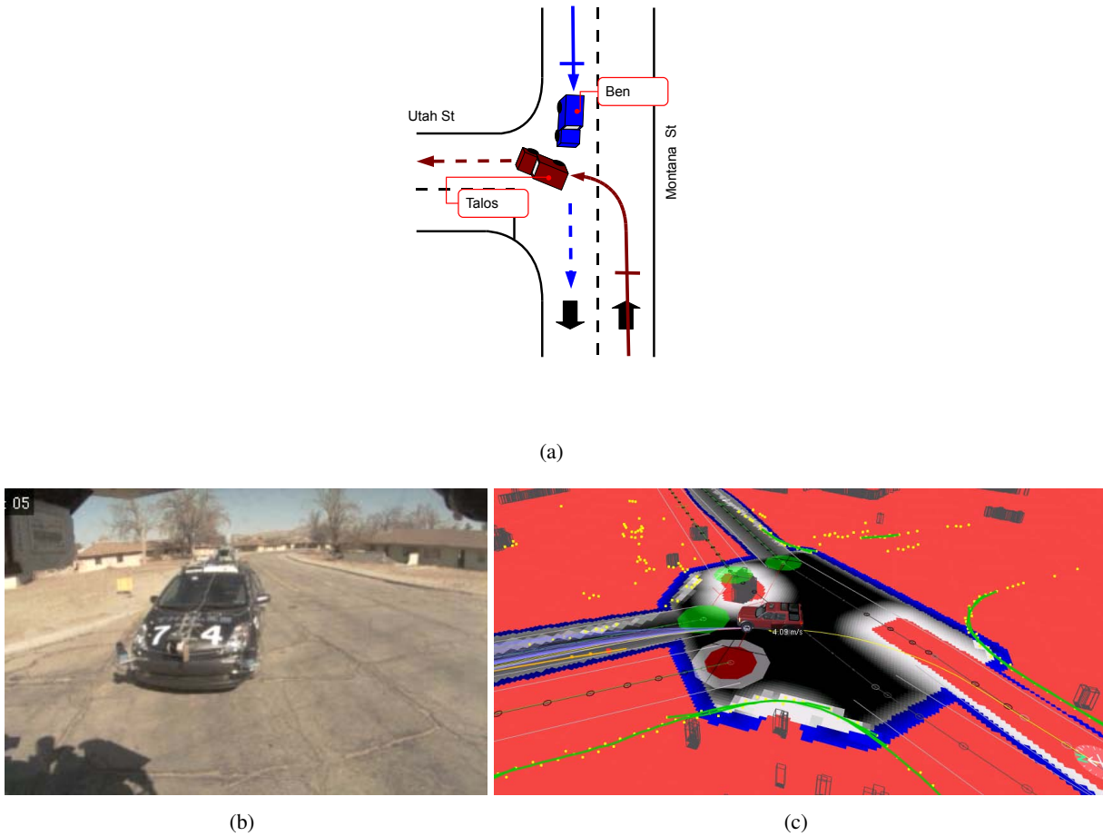
Figure 8: (a) Diagram of incident. (b) View from Talos ' right front camera. Talos ' view of the Little Ben-Talos turning near-miss. Talos yields to the velocity track of oncoming Ben (74) . Ben comes to a stop at the intersection. Talos begins motion. Ben begins to go through the intersection. Talos sees Ben as a creeping "static obstacle" and continues. Talos completes the turn. Ben stops. (c) Talos ' log visualization. Ben approaching on the right of Talos .
