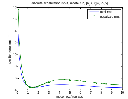
Fig. 22 Position Errors over \pm a for q = 0.01
