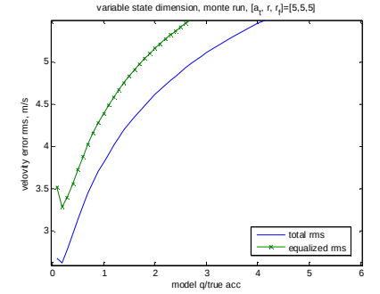
Fig. 19 Velocity Errors q_1 for q_0 = 0.01
