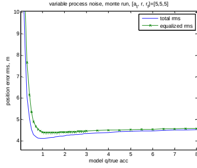
Fig. 14 Position Errors over q_1 for q_0 = 0.01
