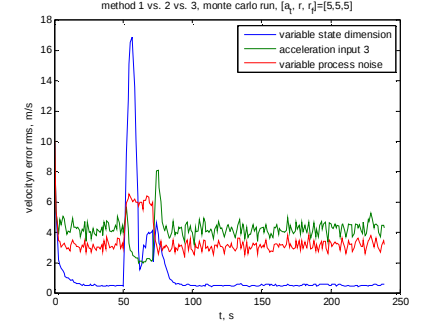
Fig. 13 Velocity Error RMS for Three Methods
