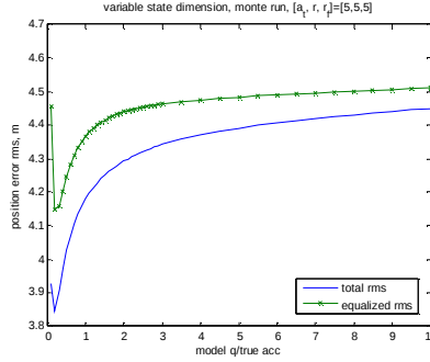
Fig. 18 Position Errors over q_1 for q_0 = 0.01
