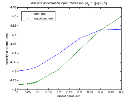
Fig. 25 Velocity Errors over q for a = \pm 5
