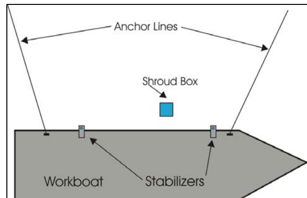
Figure 1. This is a schematic diagram showing how the support vessel is set up for a target recovery.
