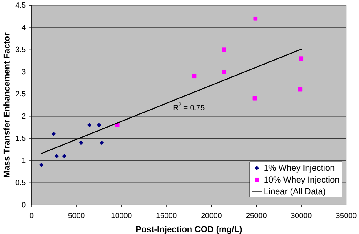
Figure 11. Correlation of mass transfer enhancement factors based on aqueous VOC concentration increases with COD concentration at Treatment Cell 2 monitoring locations following 1% and 10% whey injections.
